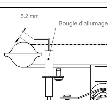
FIGURE 7 – VUE ARRIERE
