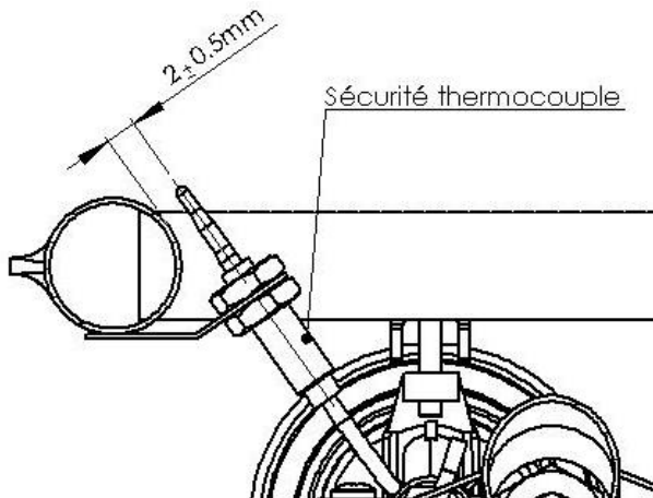
FIGURE 6 – SECURITE THERMOCOUPLE
